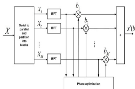
Figure 1: The structure of partial transmit sequence
