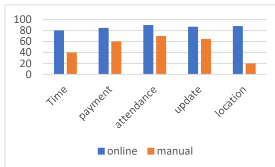
Fig 5.4 Responsive Bar-Chart
