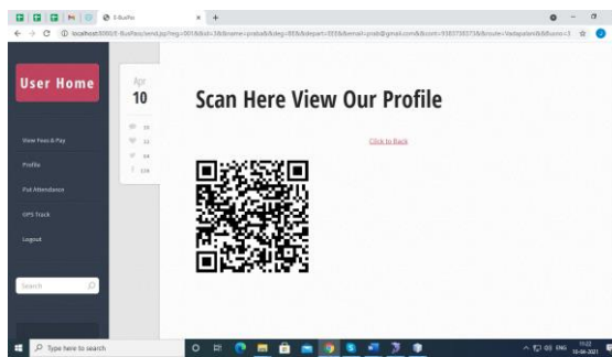
Fig 5.2 QR code
